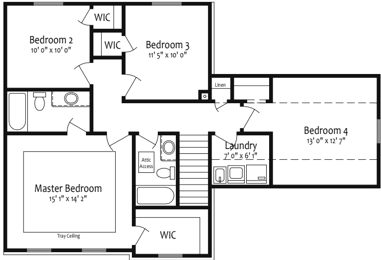
Second Floor 8' Ceilings 1019 Sq Ft
