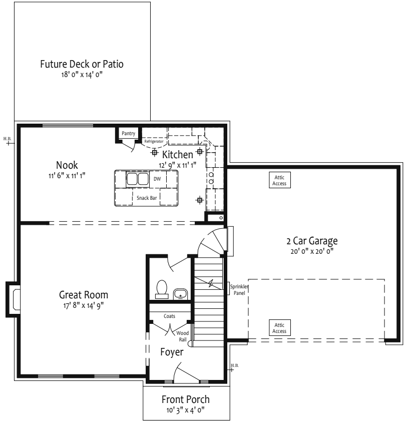
First Floor 9' Ceilings 773 Sq Ft
